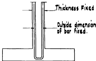
Fig. 247. Fixed Cover to Bars.
